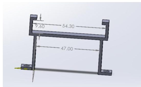
Figure 2 latest design of Battery Holder
