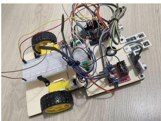
Figure 5 Assembly (Front)
