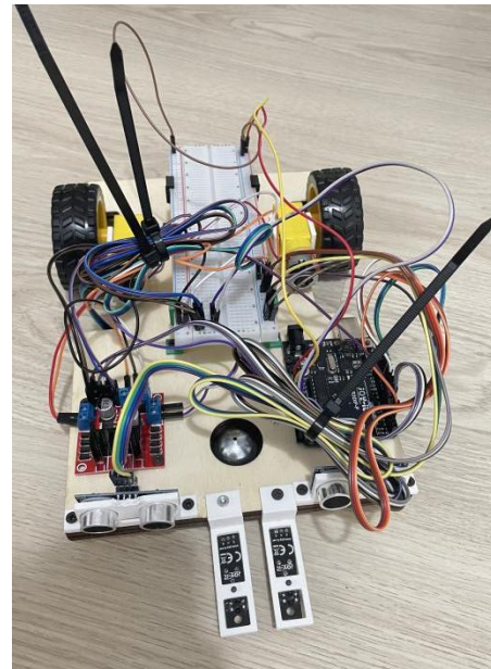
Figure 4 Assembly (Full)
