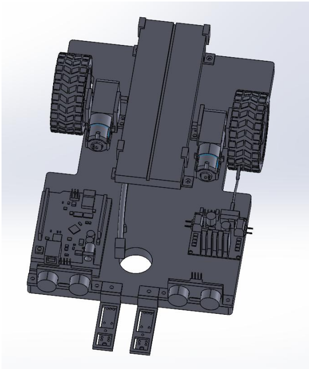
Figure 3 Assembly in Solidworks
