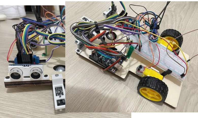
Figure 5 Assembly (Front)
